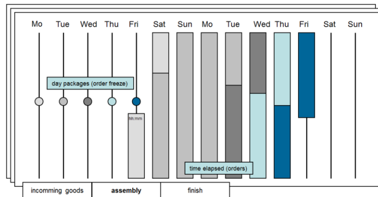
Figure 3. Concept, dispatching of orders
