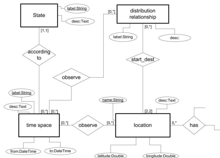
Figure 7. Part of ERM, model of problem area
