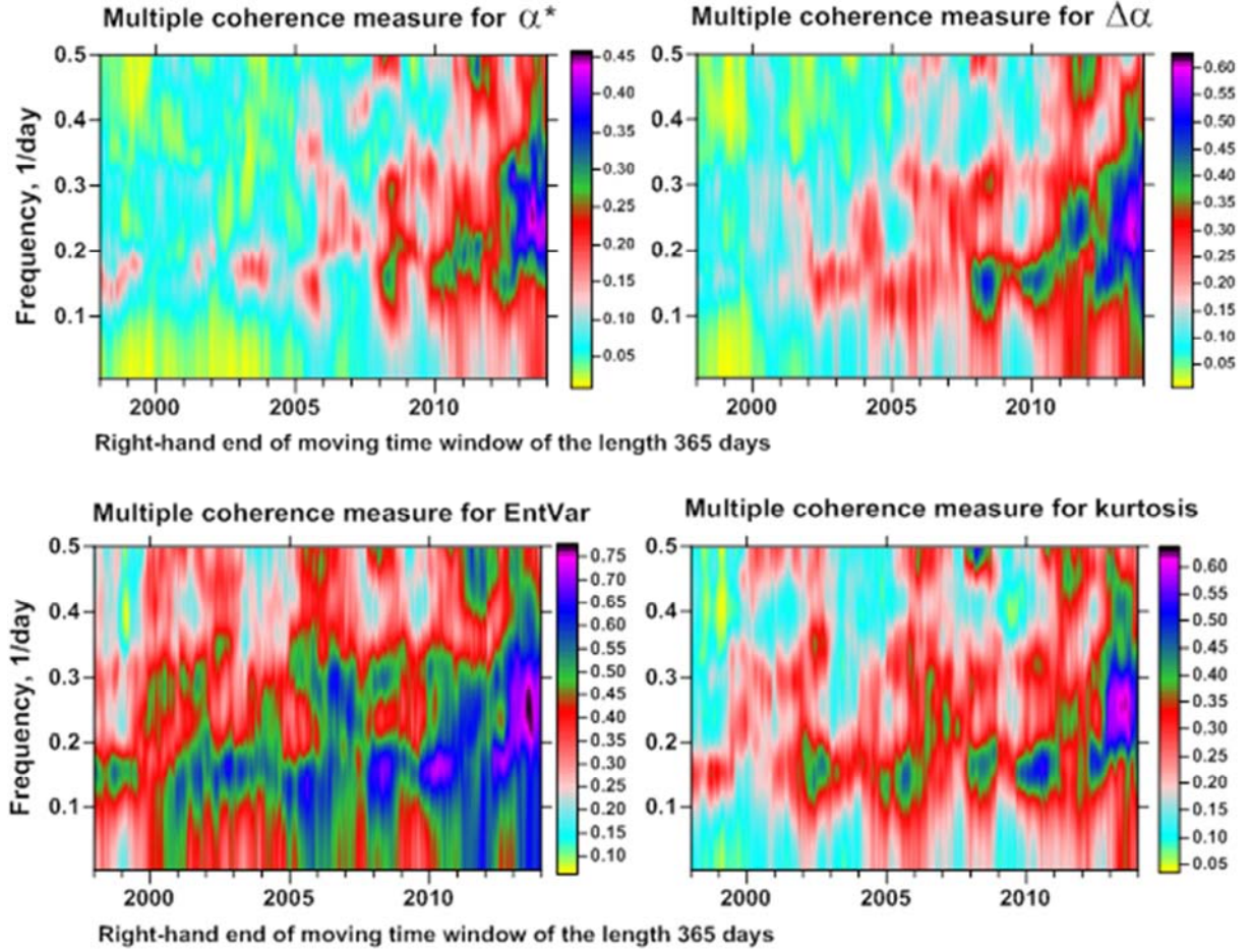
Figure 5. Time-frequency diagrams of evolution of multiple spectral coherence measure (7) for four 8-dimensional time series of daily seismic noise properties which are presented at figures 3 and 4 within moving time window of the length 365 days with mutual shift 7 days.
