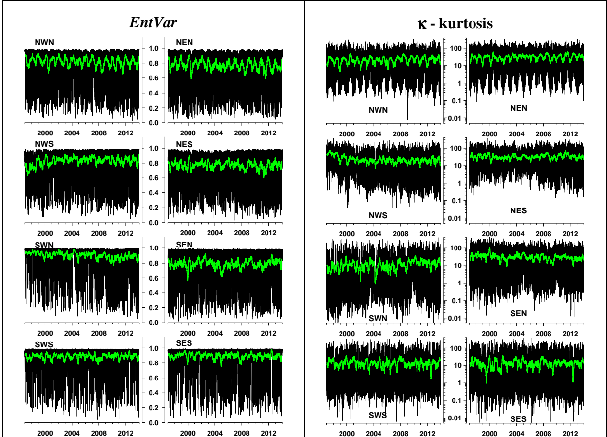
Fig.4. Daily median values of normalized entropy of variance and kurtosis of low-frequency seismic noise from 8 groups of stations presented at Fig.1. Bold green lines are graphics of running average within moving time window of the length 57 days.
