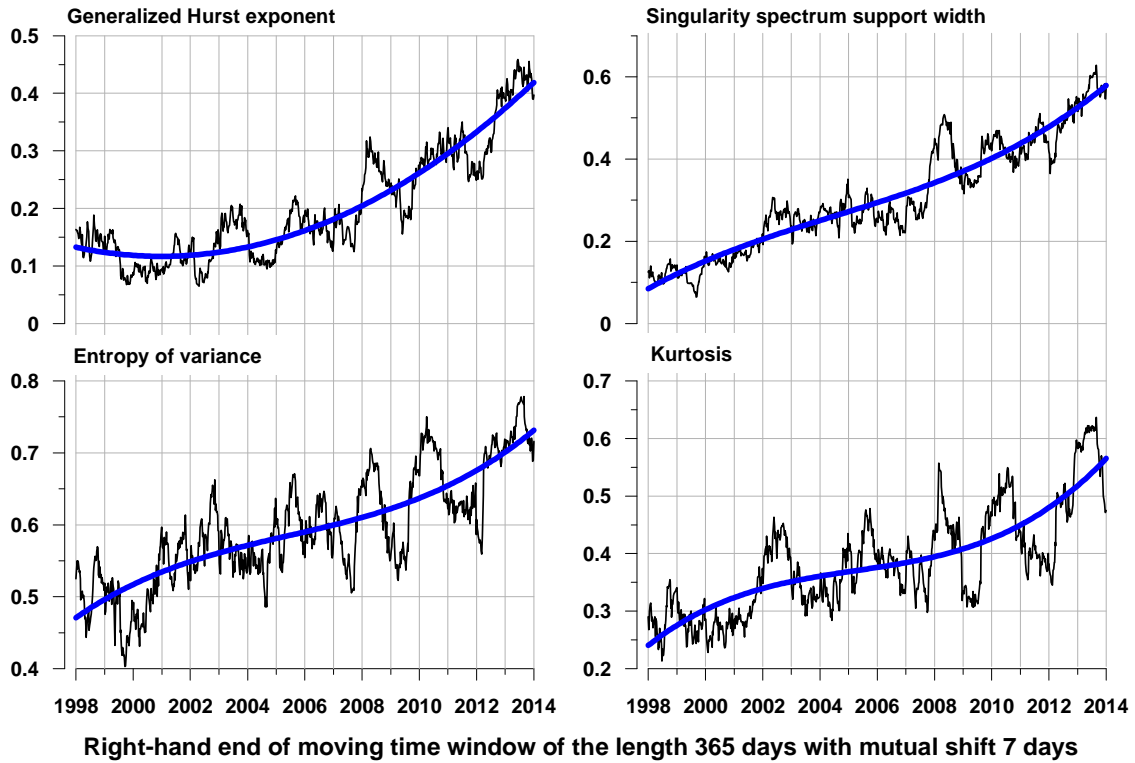
Figure 6. Maximum (with respect to frequency) values (8) of coherence measures (7) for 4 properties of low-frequency seismic noise corresponding to time-frequency diagrams at figure 5. Bold blue lines present polynomial trend of the 3 rd order.
