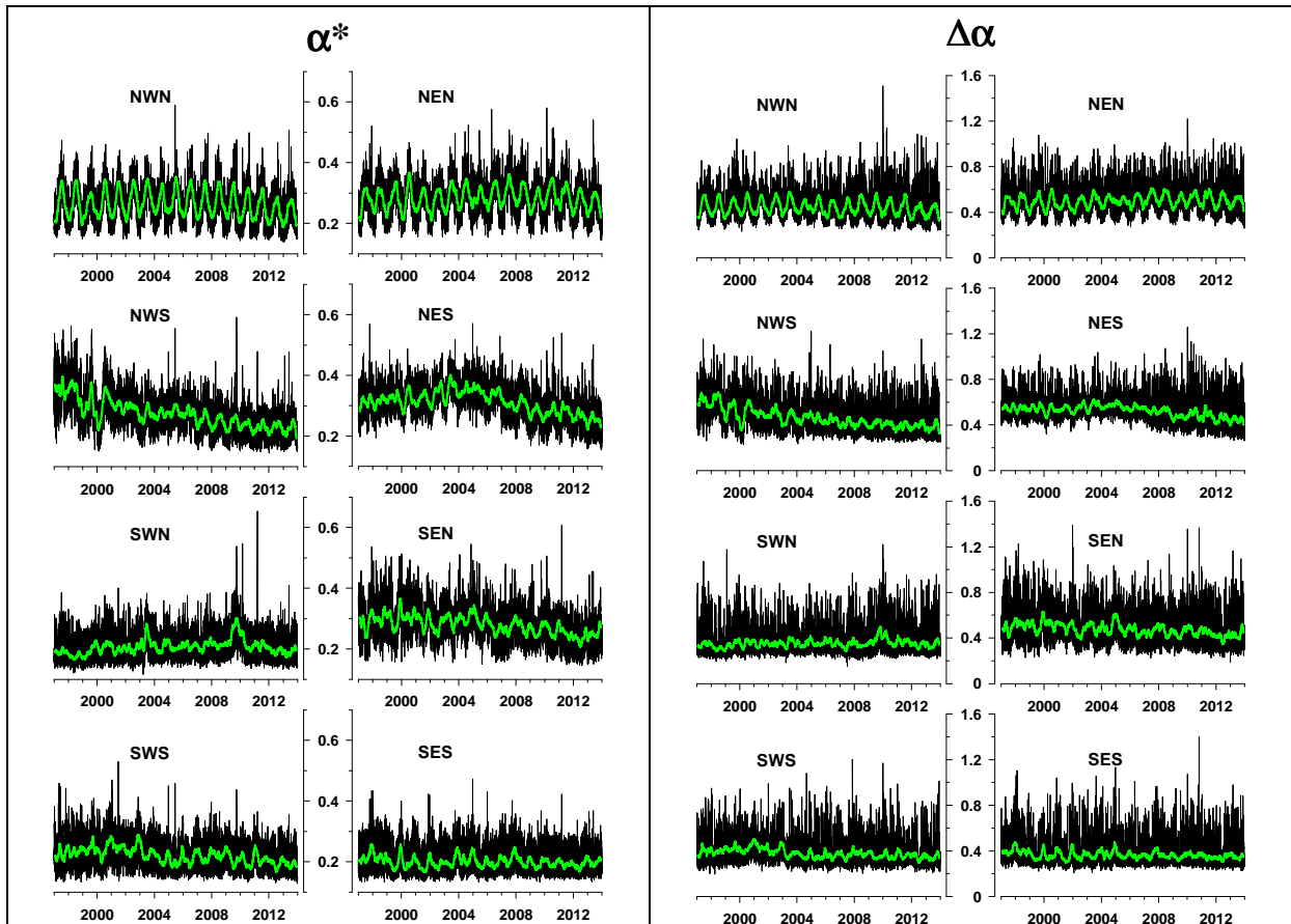
Fig.3. Daily median values of 2 multi-fractal parameters of low-frequency seismic noise from 8 groups of stations presented at Fig.1. Bold green lines are graphics of running average within moving time window of the length 57 days.
