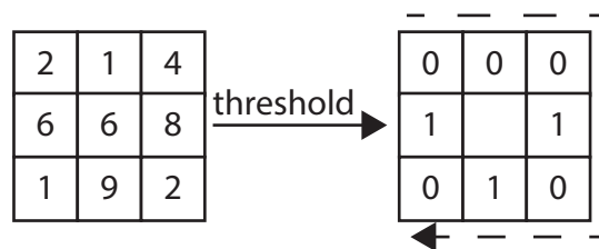
Fig. 2. Example of the LBP evaluation of a pixel with respect to its neighborhood
