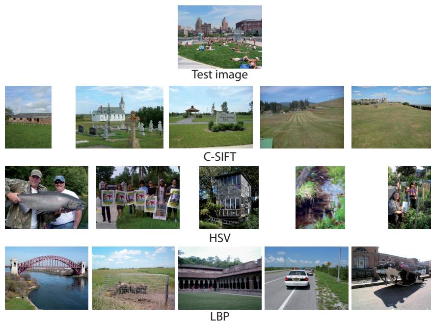
Fig. 4. Test image and the five most similar images using each visual feature (C-SIFT, LBP, HSV)
