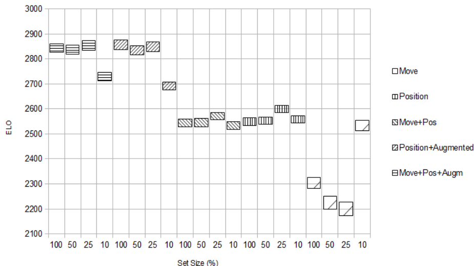
Fig. 1. Comparison of players learned from different types of preference information for four training set sizes with the square height as confidence interval.
