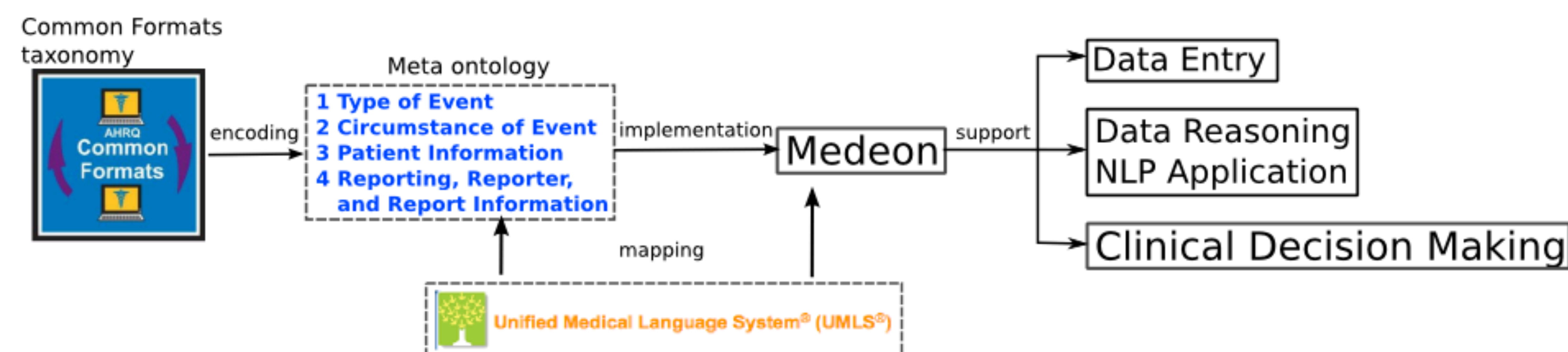
Fig 1. General framework of constructing Medeon.
