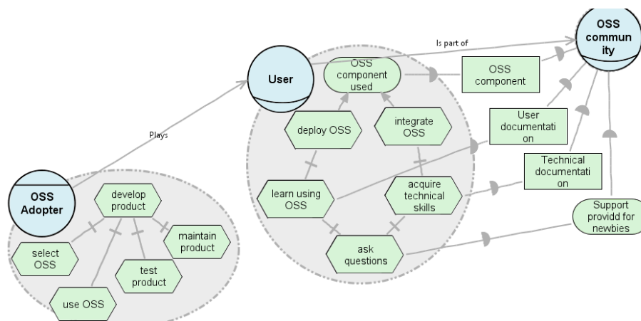
Fig. 3 Using i* plays construct to relate the OSS adopter and User
