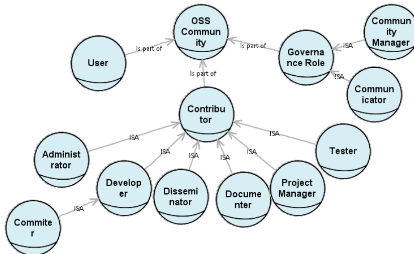
Fig. 2 OSS roles as i* roles
