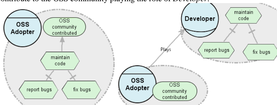
Fig. 1 OSS adoption strategy models using (right) and not using (left) i* roles 1
