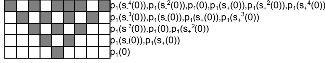
Fig. 2. Cellular automaton and corresponding Herbrand interpretations. For the states, white is 0, and grey is 1
