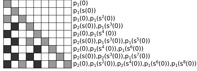
Fig. 1. Cellular automaton and corresponding Herbrand interpretations. For the states, white is 0, light grey is 1, and dark grey is 2
