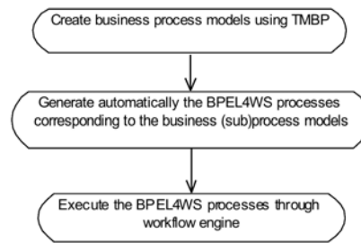
Figure 12: TMBP methodology
