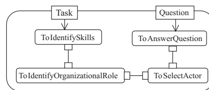
Figure 3: Candidate patterns for question answering
