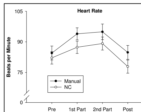
Abb. 4: Herzrate
