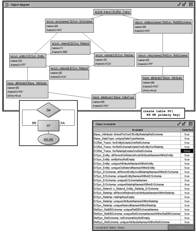
Fig. 5. Counterexample for independence of forRelshipExistsOneRelSchema.
