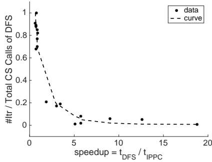
Figure 4 & Table 4: Relationship between Speedup and #Infeasible Constraints (Figure 4) and IPPC Speedup over DFS (Table 4).
