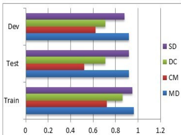
Figure 2: f-score comparison of training, testing and development set
