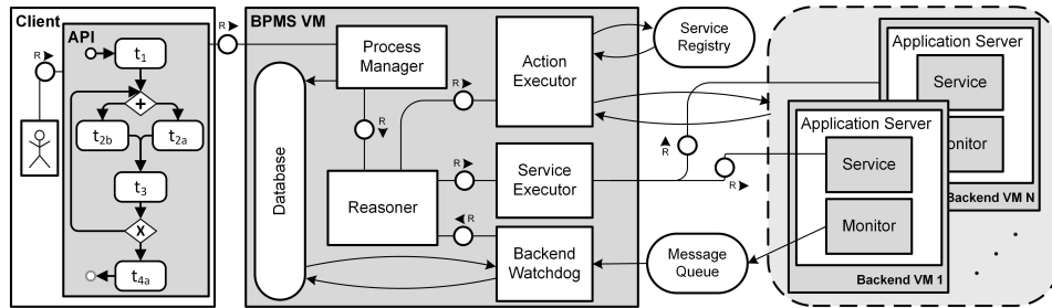
Fig. 1: ViePEP - Architecture
