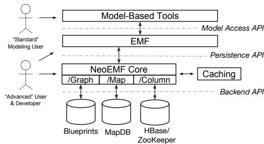
Fig. 1: NEOEMF Integration in EMF Ecosystem
