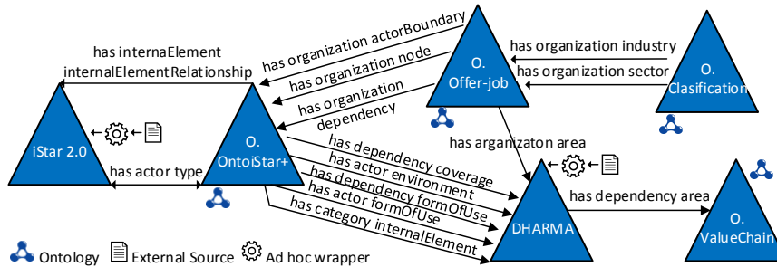
Fig. 1. DHARMA Ontology Network
