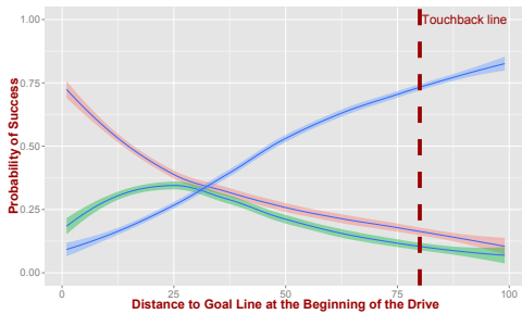
Fig. 4: A drive that starts in the opponents territory has significantly increased probability of leading to a scoring play (touchdown or field goal).
