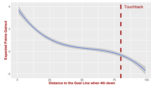
Fig. 5: The expected point benefit is positive for most of the field. The benefits become particularly tempting in the opponent's territory.
