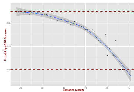
Fig.3: The overall success rate of a field goal attempt is 85% and declines with the distance from the goal.
