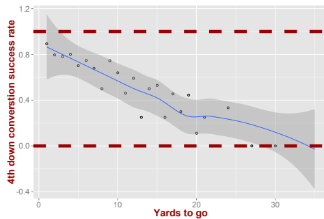
Fig.2: The fourth down conversion rate reduces with an increase of the yardage left for the first down.
