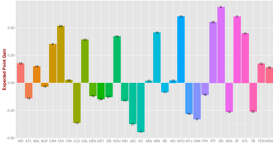
Fig. 1: Different teams have different expected point gains based on the corresponding success rates s_{2pts} and s_{kick} . On the top of each bar we also present the number of times that the corresponding team attempted a two-point conversion in our dataset.
