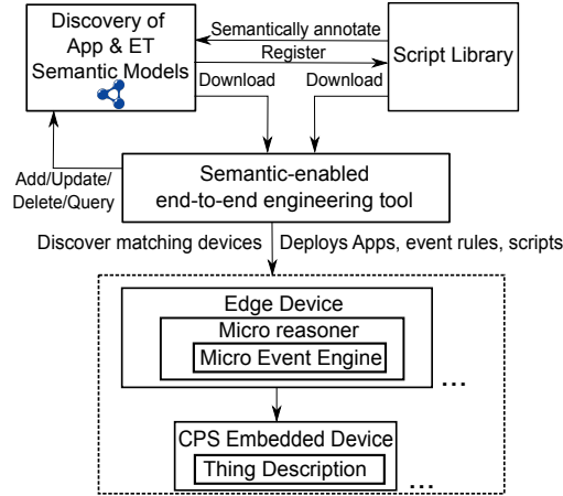
Fig. 1: The System Architecture with basic building block components
