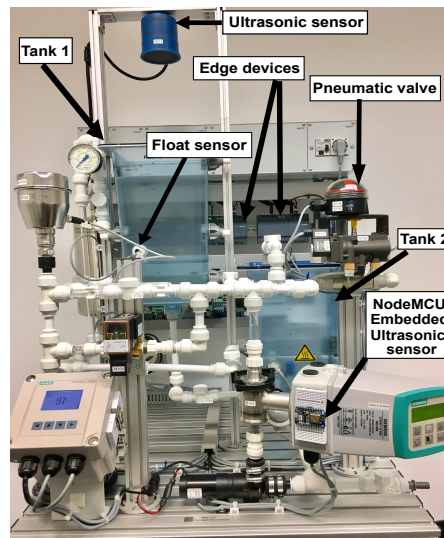
Fig. 2: Festo MPS Process Automation Workstation
