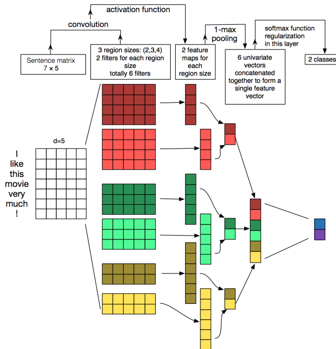
Fig. 2. Illustration of a Convolutional Neural Network architecture for sentence classification [9].
