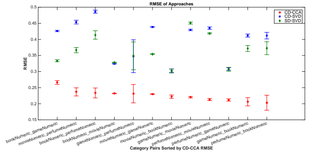
Figure 1: RMSE of algorithms on 12 Imhonet domain pairs
