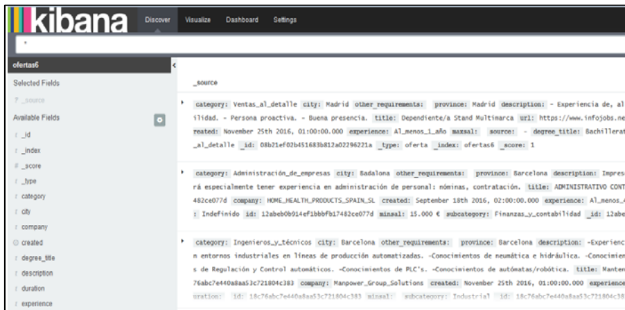
Fig. 1. Job offers stored in Elasticsearch by using Kibana (Discover interface) [7].
