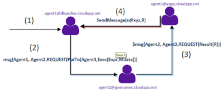
Fig. 4. Interaction between distributed agents
