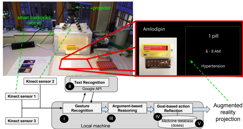
Fig. 2. Smart medicines cabinet using argument-based reasoning and an augmented reality projection. I) Gesture recognition using three Kinect cameras, one for client body capture, another for assistant personal gesture recognition, last one (Kinect sensor 2) on the top of the cabinet to recognize text from medicines boxes; II) Google API for text recognition; III) common-sense reasoning; IV) goal-based action reflection to consider human side; V) database containing doses and timing of pill intake.
