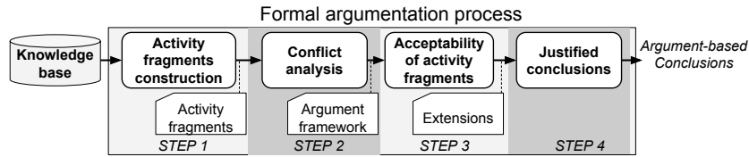
Fig. 1. Inference of an argument-based conclusion using a formal argumentation process
