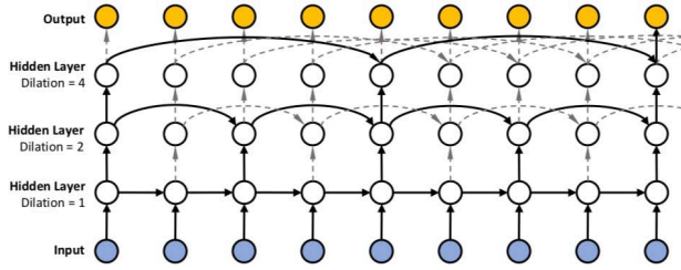
Figure 3: Structure of DRNN model. [Shiyu Chang et al., 2017]
