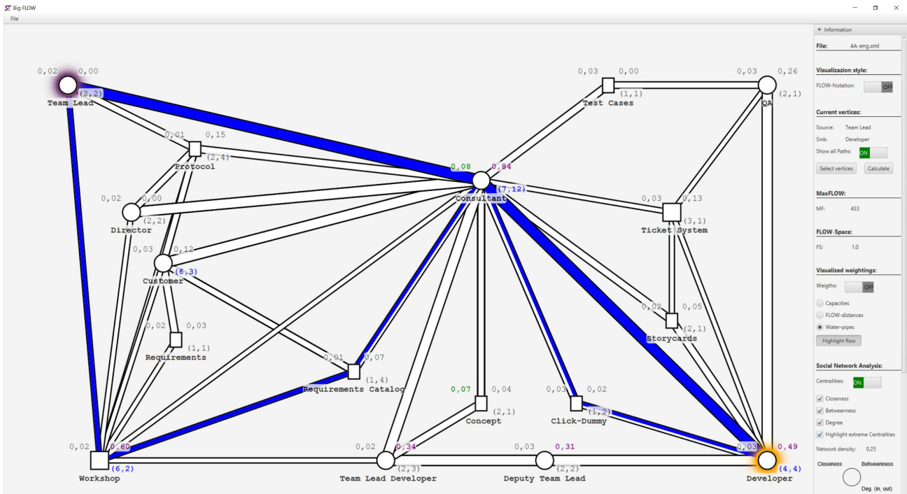
Figure 4: Screenshot of our prototype calculating the maximum information flow between the purple (source) node and the orange (receiver) node as well as common centrality measures
