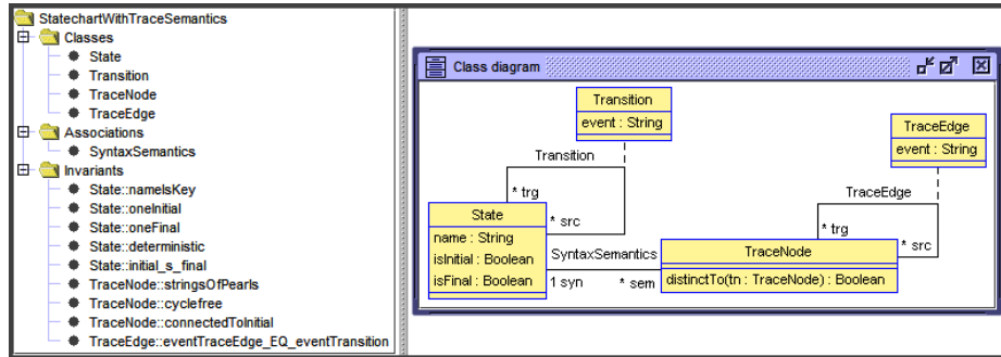
Fig. 1. A metamodel for Statecharts with trace semantics.
