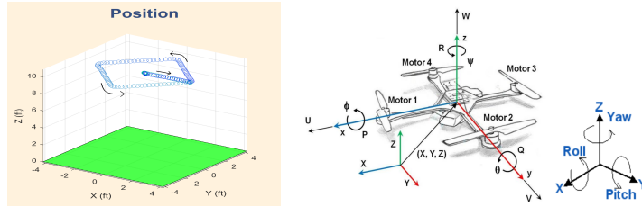
Fig. 3. Left: Simulation Path. Right: Roll , Pitch and Yaw axis of the quadcopter.
