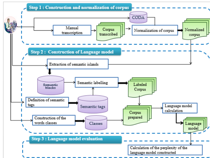
Fig. 1. Process of constructing a language model
