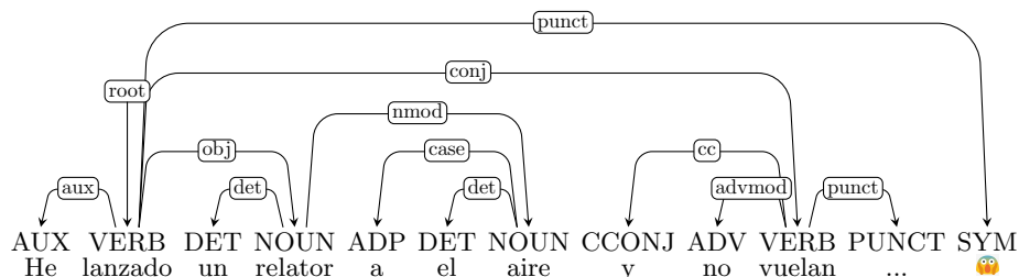
Fig. 1. Example of dependency tree.
