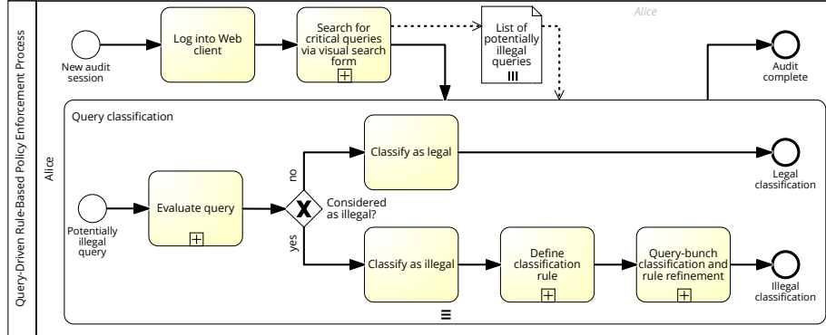
Fig. 1. Alice’s Process for Query-Driven Rule-Based Policy Enforcement
