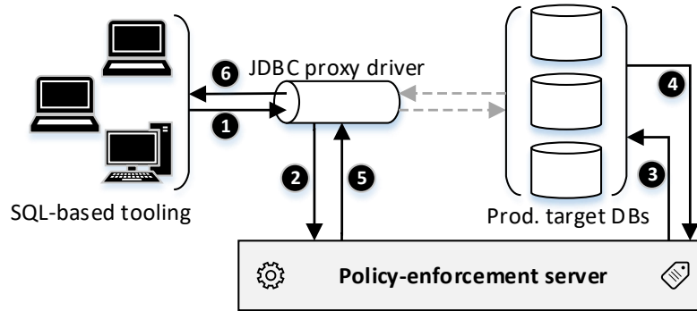
Fig. 4. Proxy driver interaction for real-time policy enforcement
