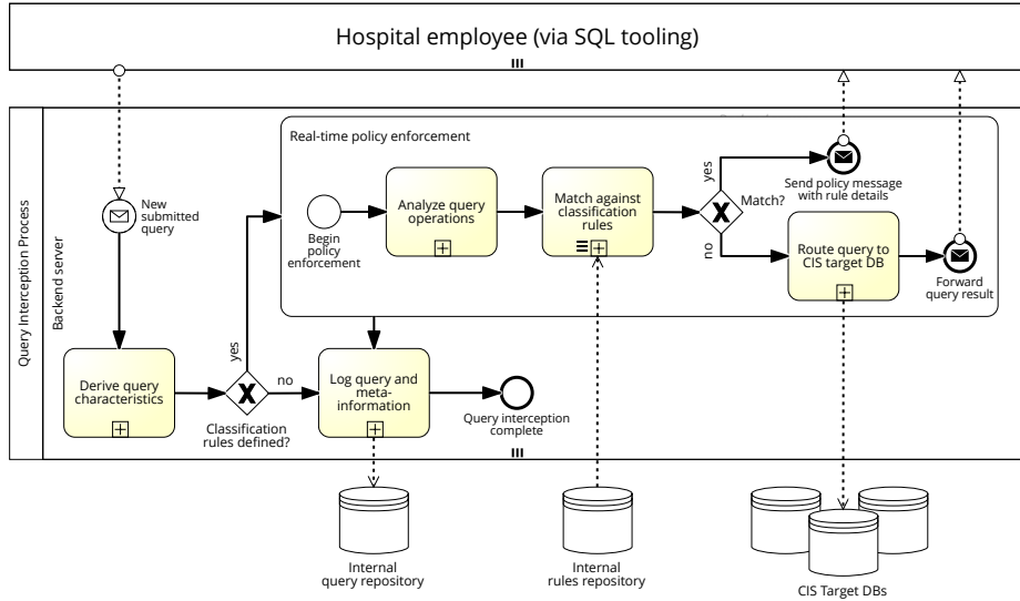
Fig. 2. Interaction of the System’s Backend Server with End-Users and Involved DBs
