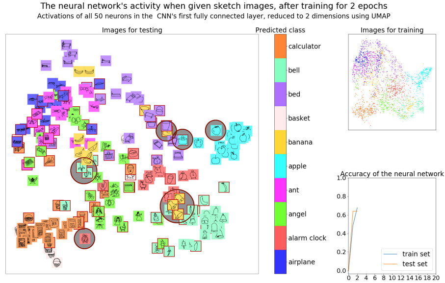
Fig. 5. Visualisation of Easy after 2 epochs. Several datapoints are highlighted with their situation type.
