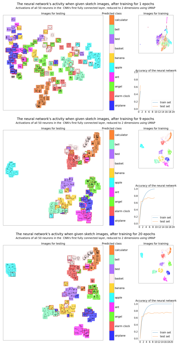
Fig. 3. Visualisation frames of epochs 1, 9 and 20 of Easy , with epoch 9 as the supposed start of overfitting.
