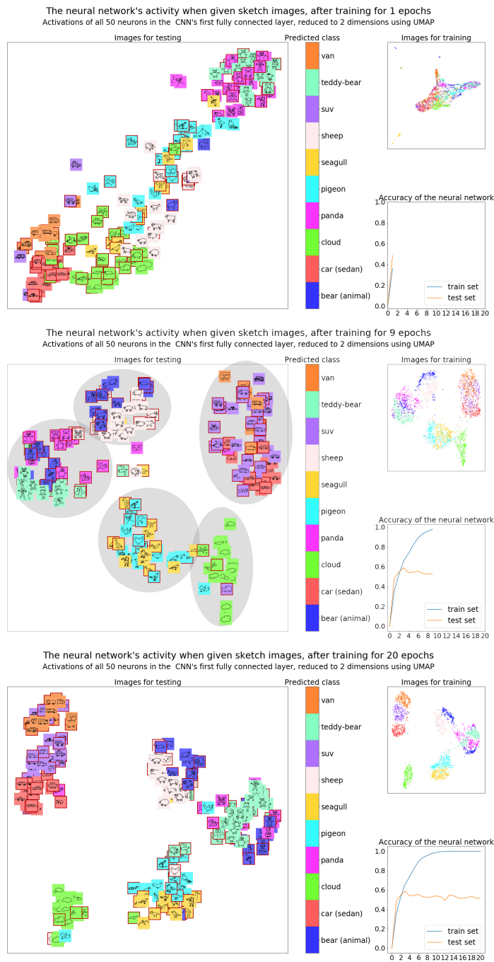
Fig. 4. Visualisation frames of epochs 1, 9 and 20 of Hard , with epoch 9 as the supposed start of overfitting. Clusters are manually highlighted for epoch 9.
