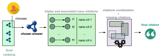
Fig. 3. Citation system for the exploitation of nano-publications.
