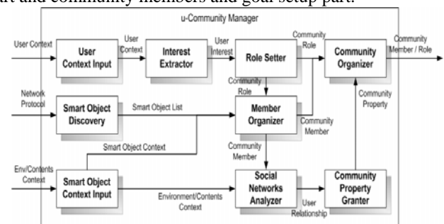
Figure 2 u-Community Manager
