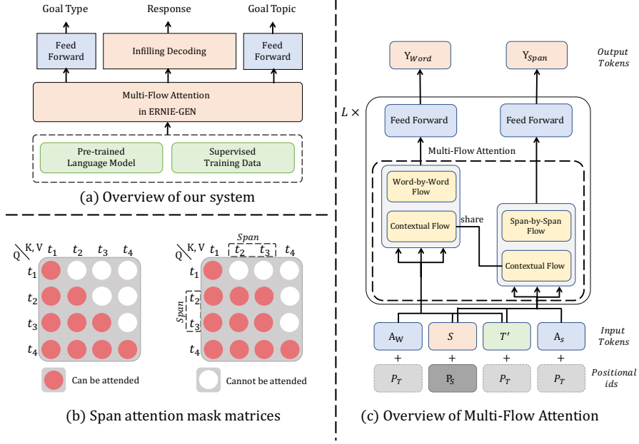
Figure 2: Illustration of methodology. (a): Overview of our system, with goal type prediction, goal topic prediction, and response generation jointly modeled in a multi-task learning manner. (b): The span attention mask matrices used in our system. (c): Overview of Multi-Flow attention in ERNIE-GEN [16], which is employed as our backbone model.
