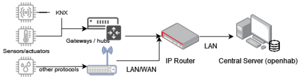
Figure 1: General architecture of the data collection system
