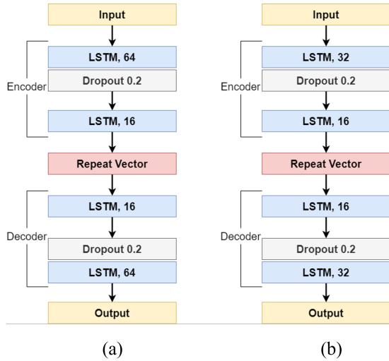
Figure 2: LSTM-Autoencoder Model Architecture
