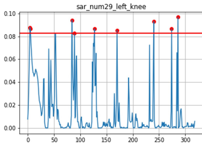
Figure 3: Anomaly Detection Result Graph
