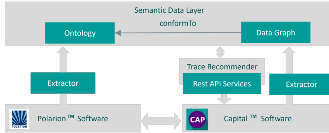
Figure 2: Traceability recommender tool - architecture.
