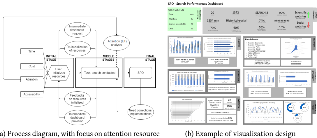
Figure 1: Proposed design for the SPD - a) Process diagram of initialization resources process, with focus on the attention one; b) Example of final SPD visualization mockup
