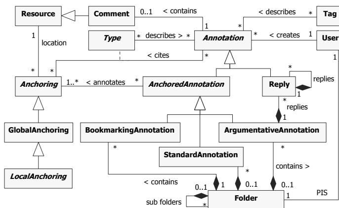
Fig. 2. UML Class Diagram of the proposed “collective annotation” concept.
