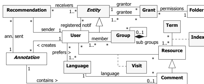
Fig. 3. Complementary UML Class Diagram for the proposed system.
