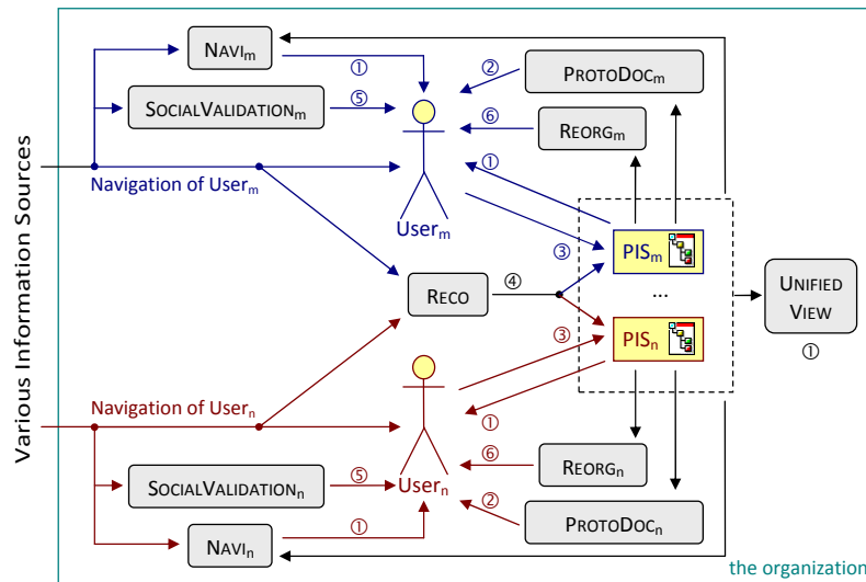
Fig. 1. Global view of the proposed architecture depicting an organization with two knowledge workers—it can be generalized to any number of users. Arrows represent data flows between the users, their PIS, and the six interconnected processes. Labels ① to ⑥ refer to the activities of the document lifecycle [1, p. 203].
