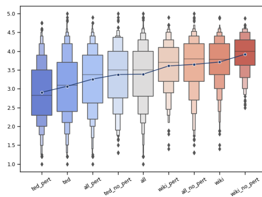
Figure 1: Overview of human judgments collected for the dataset used in sub-task 2. The plot shows the overall mean of human judgments for the whole dataset ( all ) and for respective subsets, including both coherent ( *_no_pert ) and perturbed prompts ( *_pert ).
