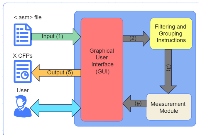
Figure 2: Architecture of the COSMIC-X86 tool prototype
