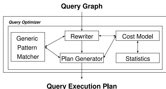
Figure 10: The architecture of the optimizer
