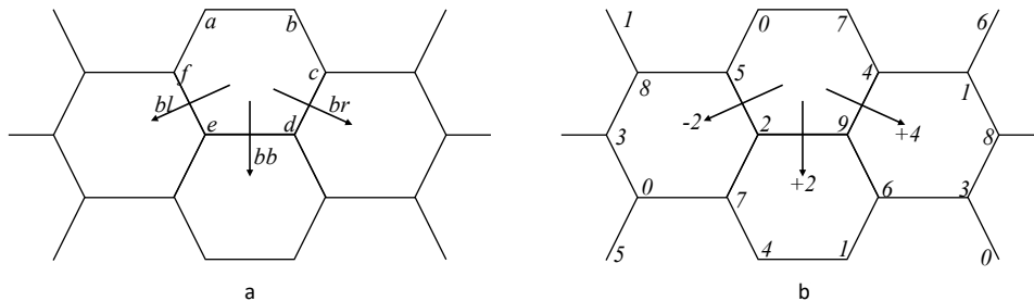
Figure 1: a. A portion of the hexagonal grid with the names associated with some of its nodes; b. L(3, 2, 1) -labeling of a portion of the hexagonal grid.
