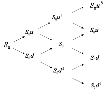
Figure 1: 3-period binomial model
