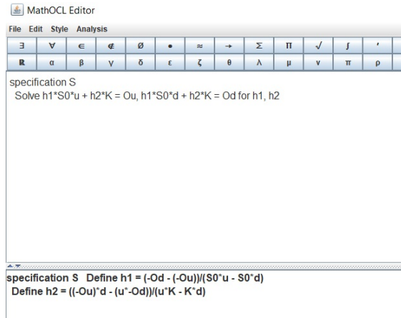
Figure 4: MathOCL model after simplification
