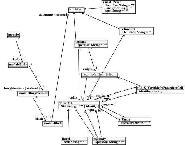
Figure 1: VB6 subset metamodel
