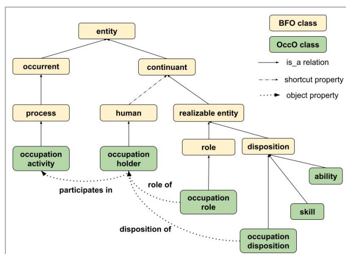
Figure 1: Key OccO Classes Extending from BFO
