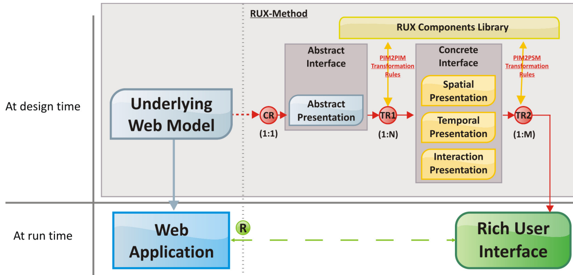
Figure 1. RUX-Method overview.
