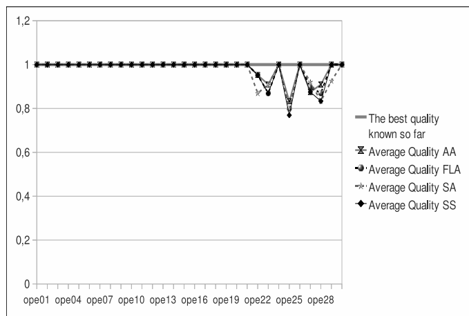
Figure 3: Best quality openstacks domain.
