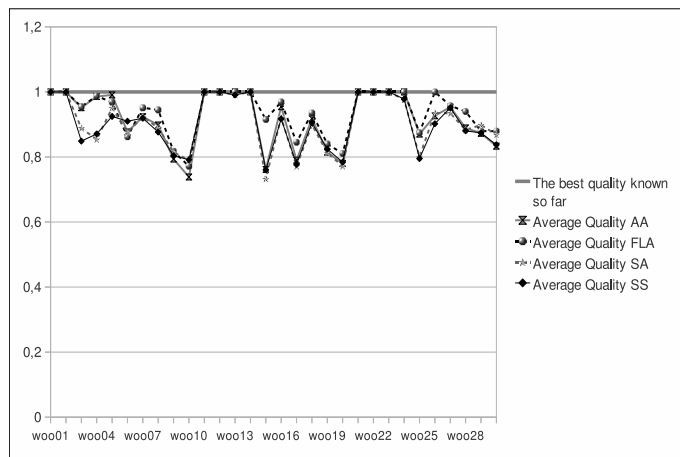
Figure 7: Best quality woodworking domain.
