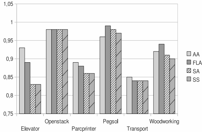
Figure 8: For each domain, each column represents a synthesis of the average quality found by means of each model. AA(Action-Action), FLA(Fuzzy-Level-Action), SA(State-Action), SS(State-State).
