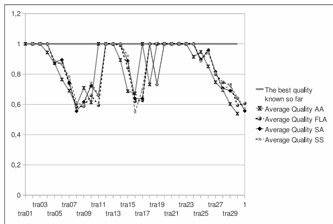
Figure 6: Best quality transport domain.
