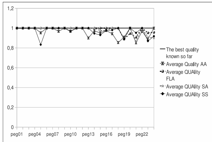
Figure 5: Best quality pegsol domain.
