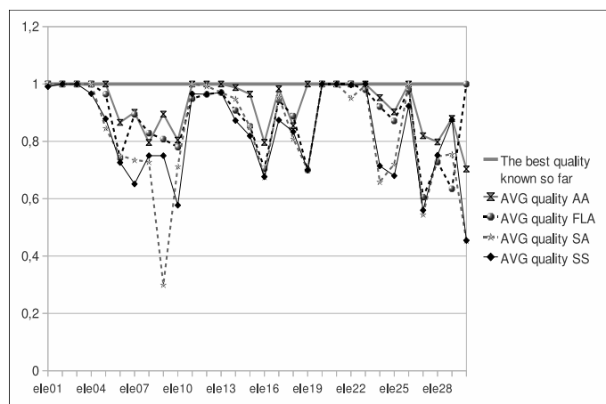
Figure 2: Best quality elevators domain,
