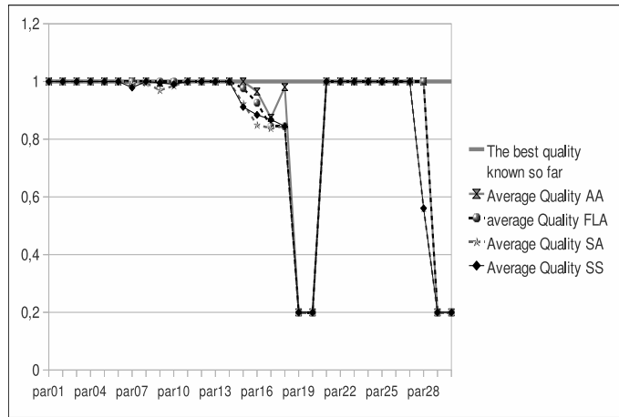
Figure 4: Best quality parprinter domain.
