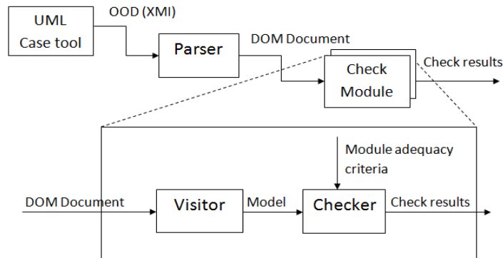
Fig. 5. The whole process of checking UML design.
