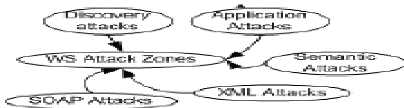
Fig. 4. Attack Zones [12]
