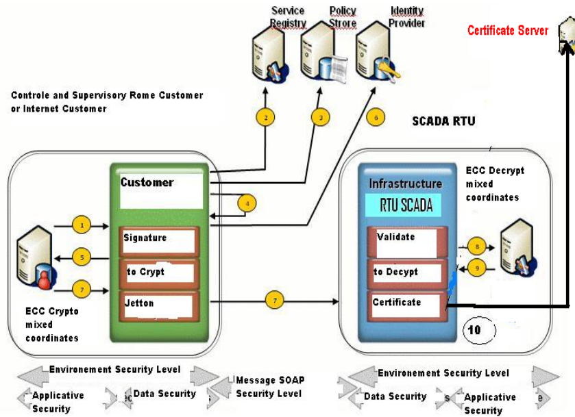
Fig.9. The Ten (10) steps of our security solution for SCADA
