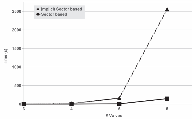
Fig. 3. Computing times of the optimization processes of the two ASP programs
